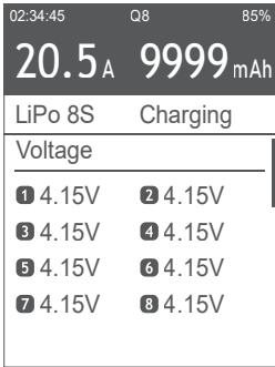
Cell voltage
